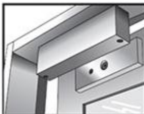
Regular Installation (outswing door)
